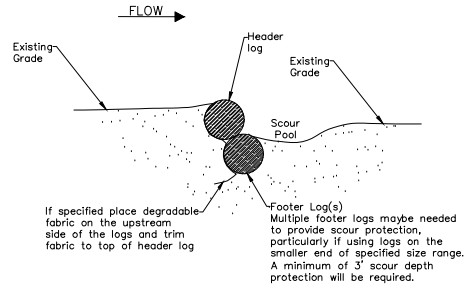
LOG DROP STRUCTURE SINGLE DROP PROFILE VIEW
