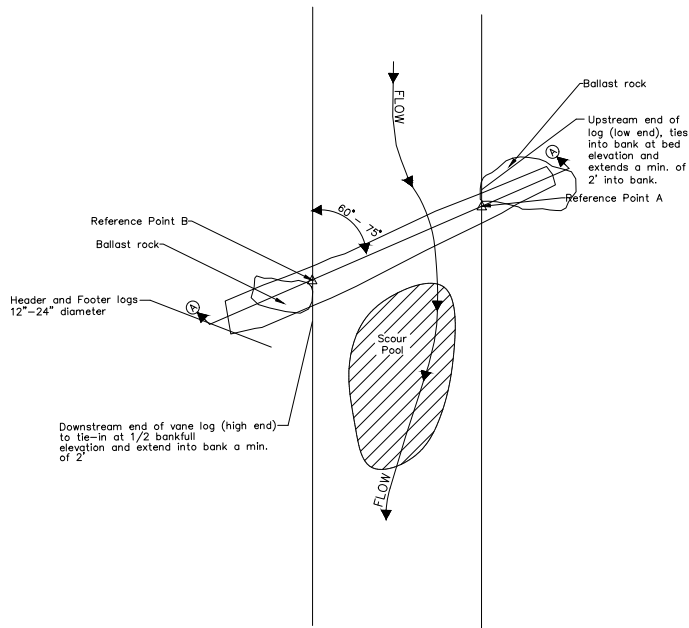
LOG DROP STRUCTURE SINGLE DROP PLAN VIEW
