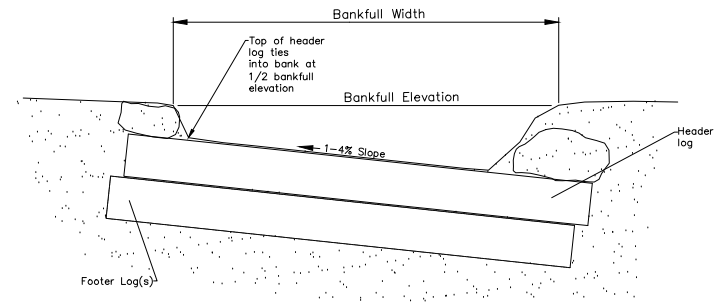
LOG DROP STRUCTURE SECTION A-A
